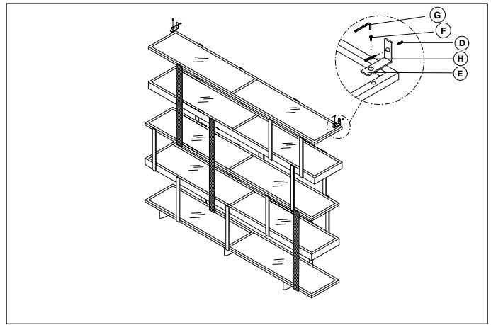
2. Install part (E) and fix the cabinet to the wall to prevent it from tipping over.
